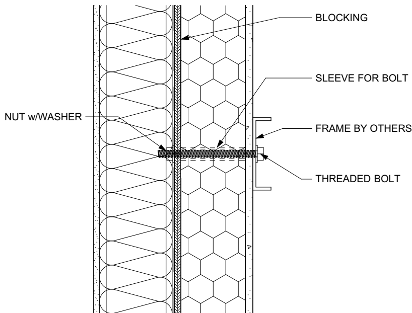
SUGGESTED ATTACHMENT DETAIL TO APPLY SIGNAGE, FIXTURES, & ETC. (OPTION TWO) (TO BE APPROVED BY E. O. R. PER PROJECT)
