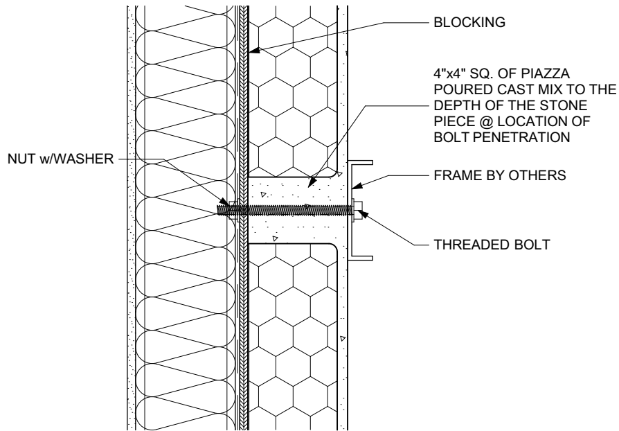
SUGGESTED ATTACHMENT DETAIL TO APPLY SIGNAGE, FIXTURES, & ETC. (OPTION ONE) (TO BE APPROVED BY E. O. R. PER PROJECT)
