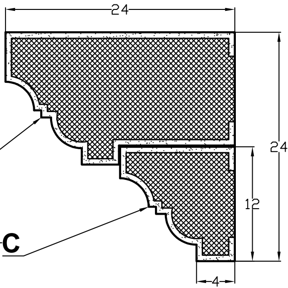
SECT. VIEW
