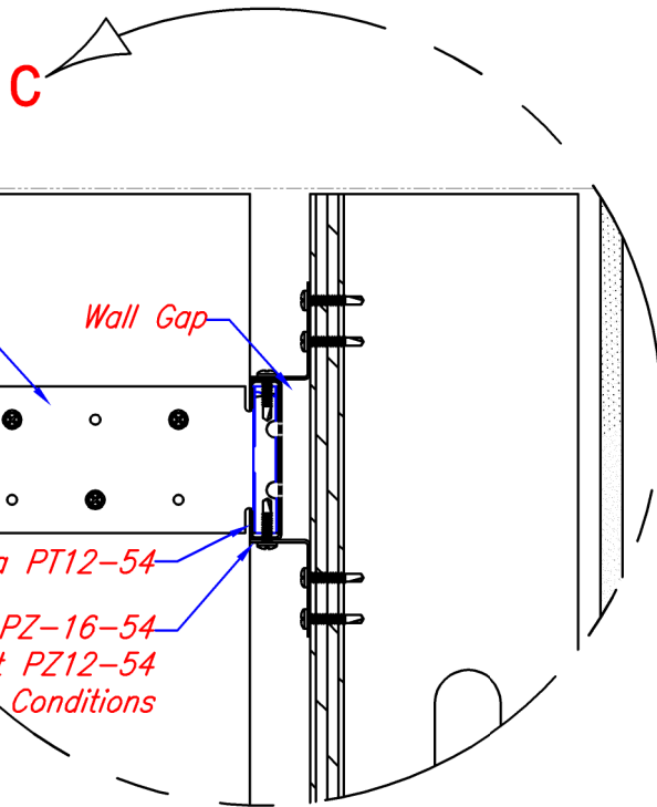
Detail C-C
